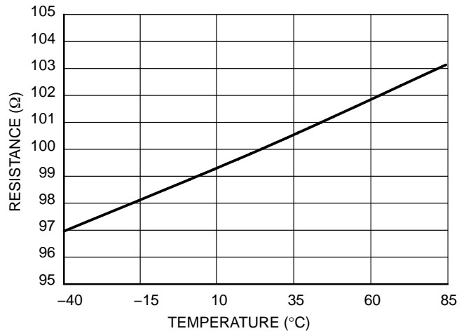
Figure 4. Resistance Over Temperature
